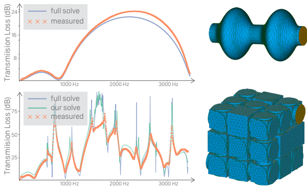
Figure 8: Double muffler and cube measured by Brüel & Kjør . Our method agrees closely with both the expensive FEM solve and the lab measurement. There is a large difference around 1600Hz, where the measurement input signal does not have sufficient power to pass through. This is caused by the wide and high transmission loss values around this region, according to the lab technicians.
