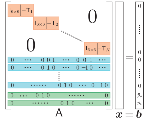
Figure 5: Linear solve of a filter assembly. The top orange part refers to the transmission matrices related to each node in the assembly. The middle blue part specifies the connection information by mapping the velocity and pressure values. The bottom two green rows are the given boundary conditions at the inlet and the outlet.
