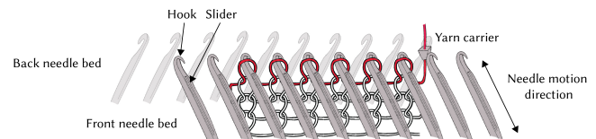
Figure 2: The needle beds in the industrial v-bed weft knitting machine
