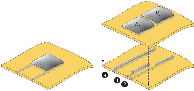
Figure 6: Two ways provided in KnitUI for connecting knitted sensors with conductive traces: left, for the single sensing unit, the conductive traces are knitted on the backside; right, due to the limited space, conductive traces are knitted on a separated fabric for designs with multiple sensing units. Conductive yarn is knitted on the bottom layer for the connection on the side but is only knitted the contact area (with the sensing unit) on the top layer to avoid shorting.
