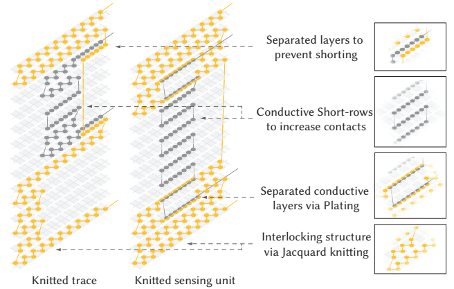
Figure 5: Needle \times time “bed view” for the sensing units and traces knits (starts from bottom). Note that we highlight each component created by knitting techniques on the right as small insets.
