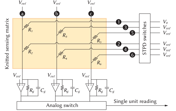
Figure 7: The modified electrical-grounding-based isolation circuit architecture for passive sensing array readout.
