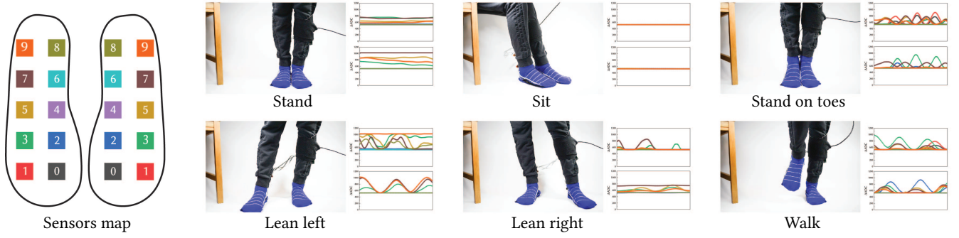
Figure 18: Sensor map and the corresponding pressure signals during six actions
