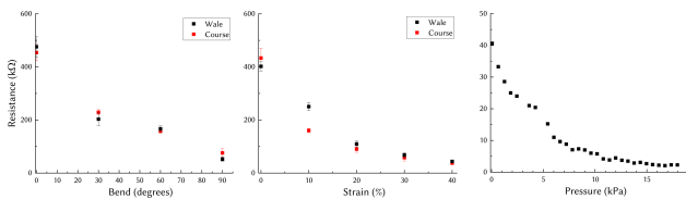
Figure 12: Resistance of a sensor at the “OFF” states of the sensors under bending (left) and stretching (middle). The resistive profile of a sensor under 40% strain along the course direction in response to the applied pressure (right).
