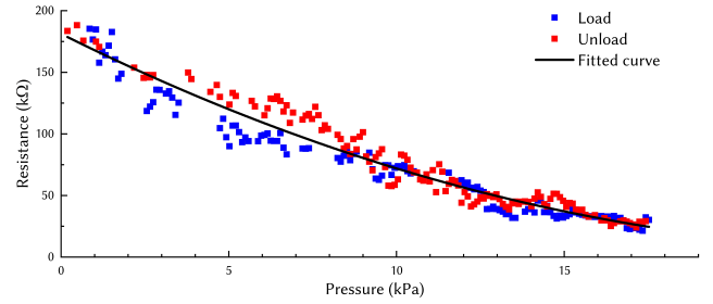
Figure 13: Continuous resistance profile of a typical knitted sensing unit in response to the load and unload of pressure
