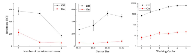
Figure 11: Resistance at the “ON” and “OFF” states of the sensors fabricated with different number of short-rows (left), sensing size (middle), and washing cycles (right).
