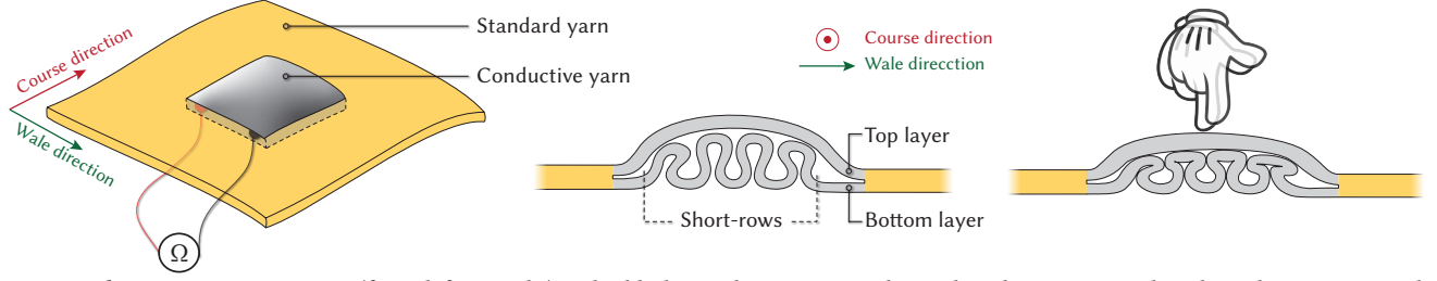
Figure 3: The sensing structure: (from left to right) a double-layered sensing unit knitted with conventional and conductive yarns; the cross-sectional view (along the wale direction) of the sensing unit, with conductive short-rows on the bottom layer to increase sensitivity; when pressure is applied, the interactions between conductive yarn loops increase, leading to the drop of resistance.
