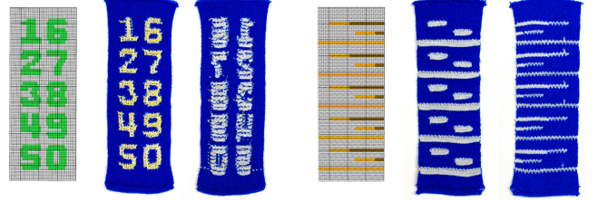
Figure 10: An example of Numpad designed by KnitUI interface: left, the patch with 10 separated sensors (the front and back of the corresponding knitted result), and right, the design of knitted traces to connect the sensors with the readout circuit and the corresponding fabricated result.
