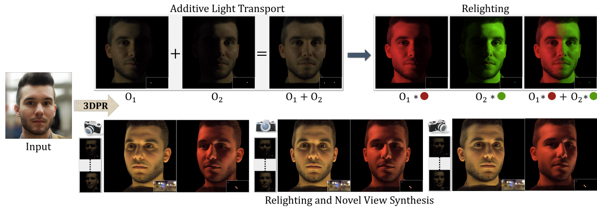
Fig. 1. We present 3DPR, a monocular 3D portrait relighting method that can synthesize novel views under desired illumination. Given a monocular input image, 3DPR predicts a reflectance basis in the form of One-Light-At-a-Time (OLAT) images of the subject (top row). By linearly combining the OLAT basis based on given HDRI map, the subject can be placed in novel relit environments (bottom row). Moreover, the OLATs can be rendered for a desired novel camera viewpoint, facilitating 3D-consistent portrait relighting.
