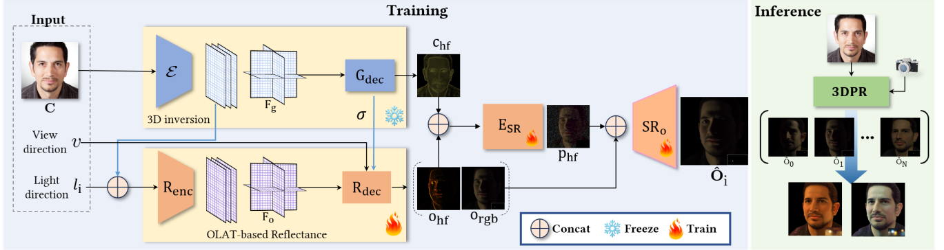
Fig. 3. Given one portrait image C , 3DPR renders the subject from a novel viewpoint under new lighting. Left: During the training stage, C is first fed into the 3D-aware encoder \mathcal{E} [Yuan et al. 2023] to produce tri-planar features F_g , concatenated with a given light direction l_i . Then, the concatenated features are fed into the Reflectance Encoder R_{enc} and Reflectance Decoder R_{dec} to render a low-resolution OLAT image o_{rgb} and high-frequency reflectance features o_{hf} . We further combine o_{hf} with the corresponding appearance features c_{hf} , to be fed into SR Encoder E_{SR} to obtain fused high frequency features p_{hf} . At the end, the OLAT Super-Resolution network SR_o produces a high-resolution OLAT image \hat{O}_i . In our architecture, we use pre-trained networks [Chan et al. 2022] for StyleGAN and G_{dec} and keep these modules frozen, and only train R_{enc} , R_{dec} , E_{SR} and SR_o on light stage dataset. Right: During inference, 3DPR takes a single portrait image, view and light direction as input, and synthesizes OLATs, which are then linearly combined for novel illumination.
