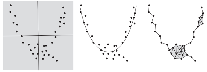
(a) Linear model (b) Non-linear model (c) Piecewise linear model
