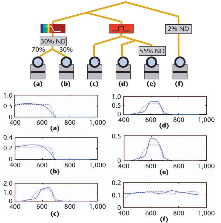
12 Plots of (I \cdot x) versus \lambda nanometers for a complex camera. Dashed lines are the specification, solid lines are the final design; for a good design, these are close in both magnitude ( I ) and shape ( x ). The design tool independently matched each spectral efficiency curve close to the specification, taking into account imperfections in the actual filters.
