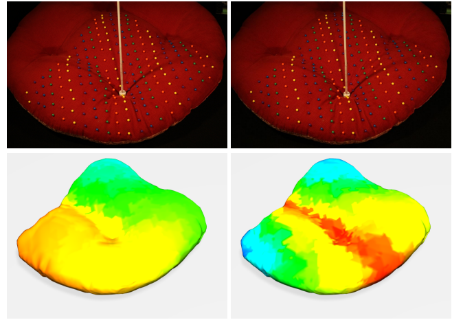
Figure 3: Two examples of a deformed pillow with color-coded Young's modulus ('blue' is low, 'red' is high), which varies both as a function of location and the local strain. Probe pressure was higher on the right.
