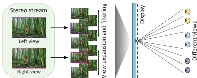
Figure 2: Our method takes a 3D stereo stream as an input, and performs a view expansion together with an antialiasing filtering to obtain a correct input for an automultiscopic display. ("Sintel" © by Blender Foundation)
