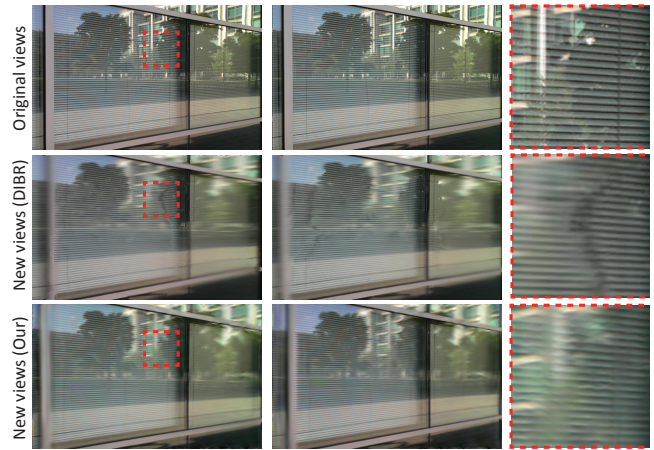
Figure 6: Transparent and highly reflective objects are very challenging for any depth estimation and view synthesis methods. The figure shows the input images (top) and views that were generated using depth image-based technique (middle) and our method (bottom). The technique that relies on the depth estimation fails to reconstruct highly reflective and transparent objects.
