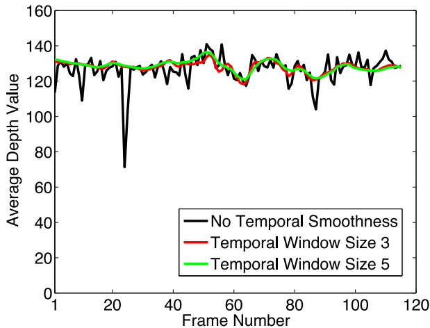
Fig. 17. The average depth values for each frame of a synthetic sequence, when using different temporal window sizes. While without temporal smoothness the scene experiences sudden changes of depth, the depth changes are much smoother when temporal smoothness is applied.
