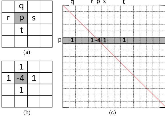
Fig. 4. Construction of matrix A of the Poisson equation. (a) An example 4 \times 4 image, showing a sample pixel p and its neighbors. (b) The coefficients of (3) for pixel p . (c) The non-zero values in A for the row corresponding to pixel p .
