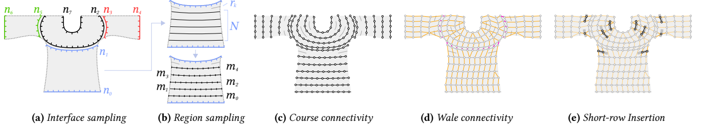
Fig. 10. Illustration of the steps of our sampling algorithm: (a) optimizing stitch numbers at region interfaces (Sec. 6.1), (b) optimizing course number, short-row densities and stitch numbers in each region (Sec. 6.2), (c) creating stitch courses (Sec. 6.3.1), (d) pairing stitches between adjacent courses across interfaces (Sec. 6.3.2) and within regions (Sec. 6.3.3), and (e) generating short-row stitches (Sec. 6.4).
