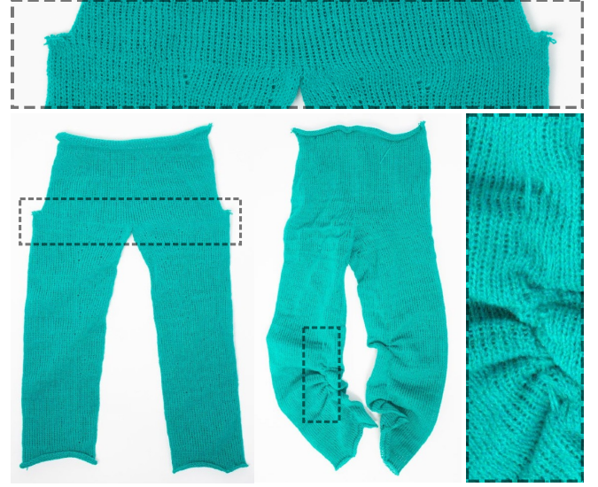
Fig. 17. Example of knitting failures due to failing needle transfers: the left example failed at large decreases above the crotch due to non-ideal schedule alignments; the right example had catastrophic failures due to overlapping loop transfers during shaping transfers.
