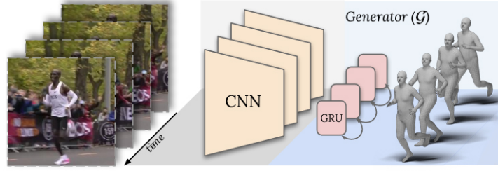
Fig. 4. VIBE Architecture [35].
