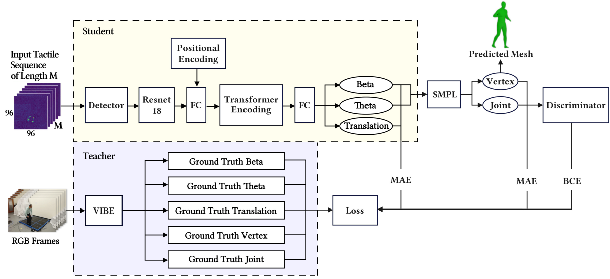
Fig. 3. Architecture of CAvatar. Video from cameras is employed solely during the training phase, serving as a "supervisor" for the tactile signals. However, it is important to note that these camera videos are not utilized during actual practice or application.
