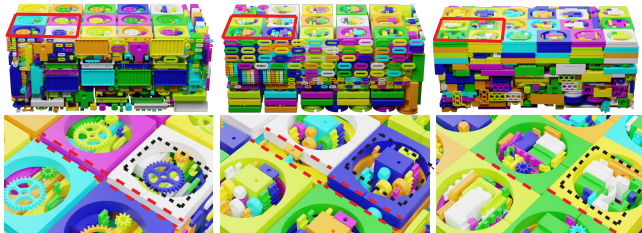
Fig. 15. Comparison between our algorithm and commercial software on PIECES. Left: Netfabb. Middle: Fabbplot. Right: Our algorithm. The bottom row shows in-focus views of the result. Both Netfabb and Fabbplot produce wide gaps between objects as highlighted with red dashed line. Also notice our algorithm is able to fill void space more efficiently as shown in the black square.
