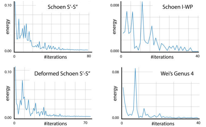
Fig. 7. Convergence of edge length optimization. We demonstrate convergence for the 4 TPMS with the longest optimization times, which use different FBVs: Schoen I-WP uses a prism, while the others use an AAB.
