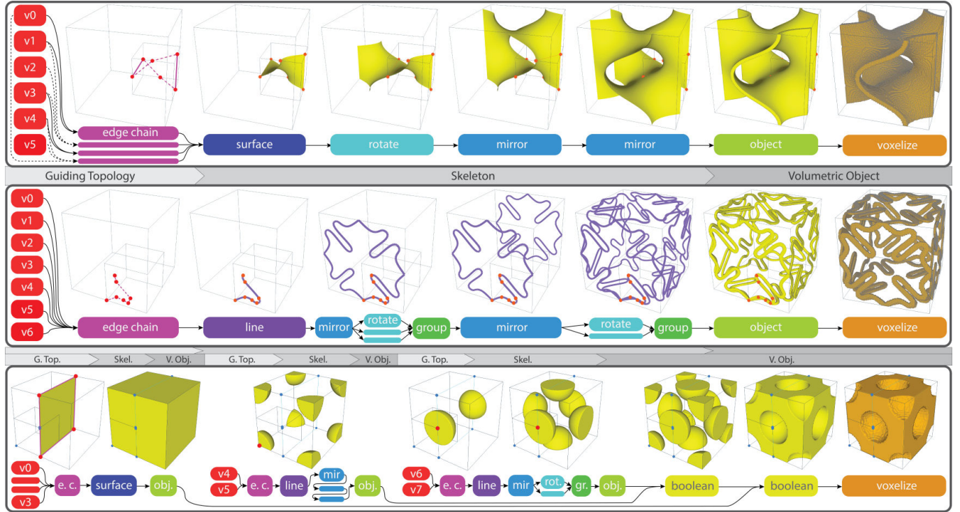
Fig. 2. Metamaterial construction. Our graphs succinctly create structures based on (top) a recently-discovered TPMS [Chen and Weber 2021], (middle) auxetic curved beams [Jenett et al. 2020], and (bottom) a face-centered cubic solid [Lu et al. 2017]. Edge chains can be smooth (dashed) or non-smooth (solid).
