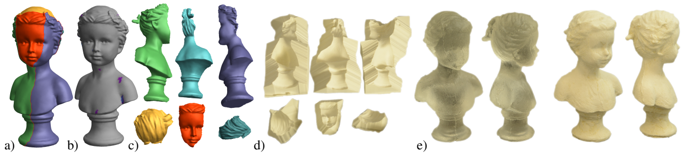
Figure 1: To fabricate a mesh (possibly acquired by laser scanning) in a molding process, we decompose the shape into parts that largely satisfy molding constraints. The resulting constraint violation (b) can be removed by deformation (c). A reusable multi-piece mold can be produced from the final mesh by CNC milling (d) and physical copies can be produced by mold casting in different materials like resin (left) or plaster (right) (e). The buste model is provided by the AIM@SHAPE Shape Repository.
