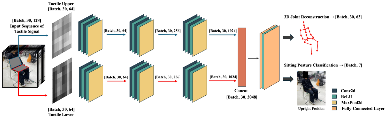
Figure 3: Model architecture for 3D posture reconstruction and classification
