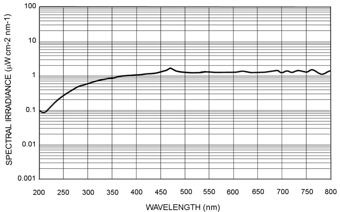
Figure 3-3: Spectral Irradiance 50 cm from the light source.
