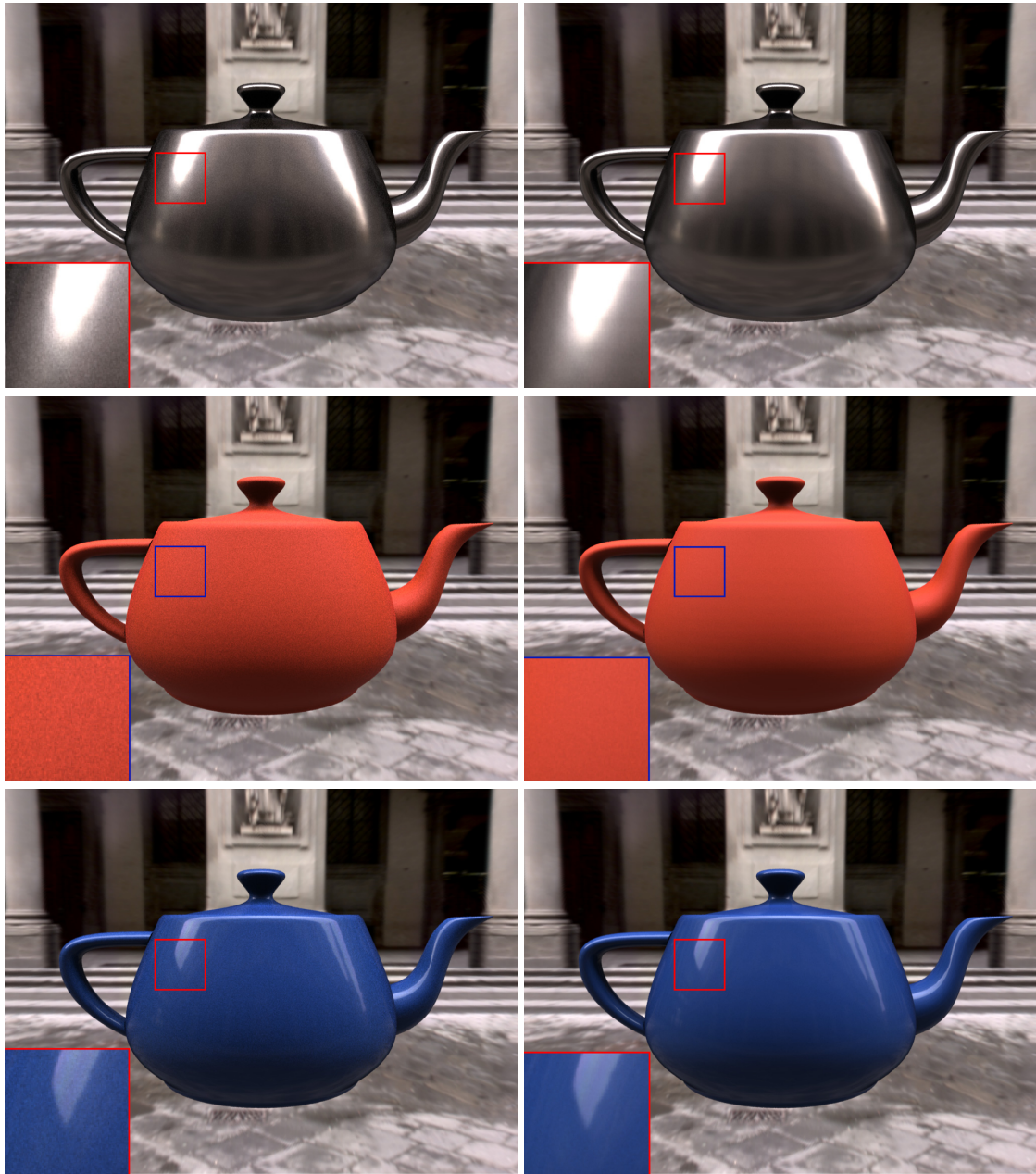
Figure A-2: Renderings under complex natural illumination. Importance sampling is used to decrease the noise: first column: 100 samples, second column: 1000 samples.
