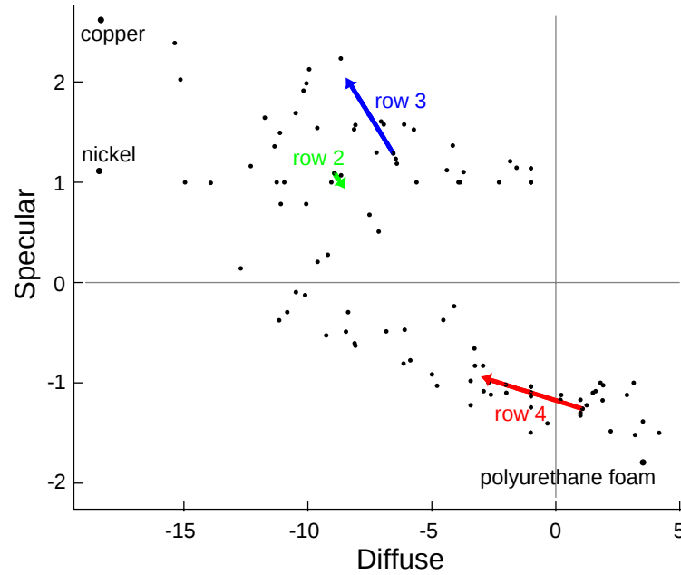
Figure 5-2: Diffuseness trait vs specularness trait. Observe that the diffuseness and specularness traits exhibit a weak inverse correlation. The green, blue, and red vectors denote projections of the BRDF interpolations shown in the second, third, and fourth rows of Figure 5-6 respectively.
