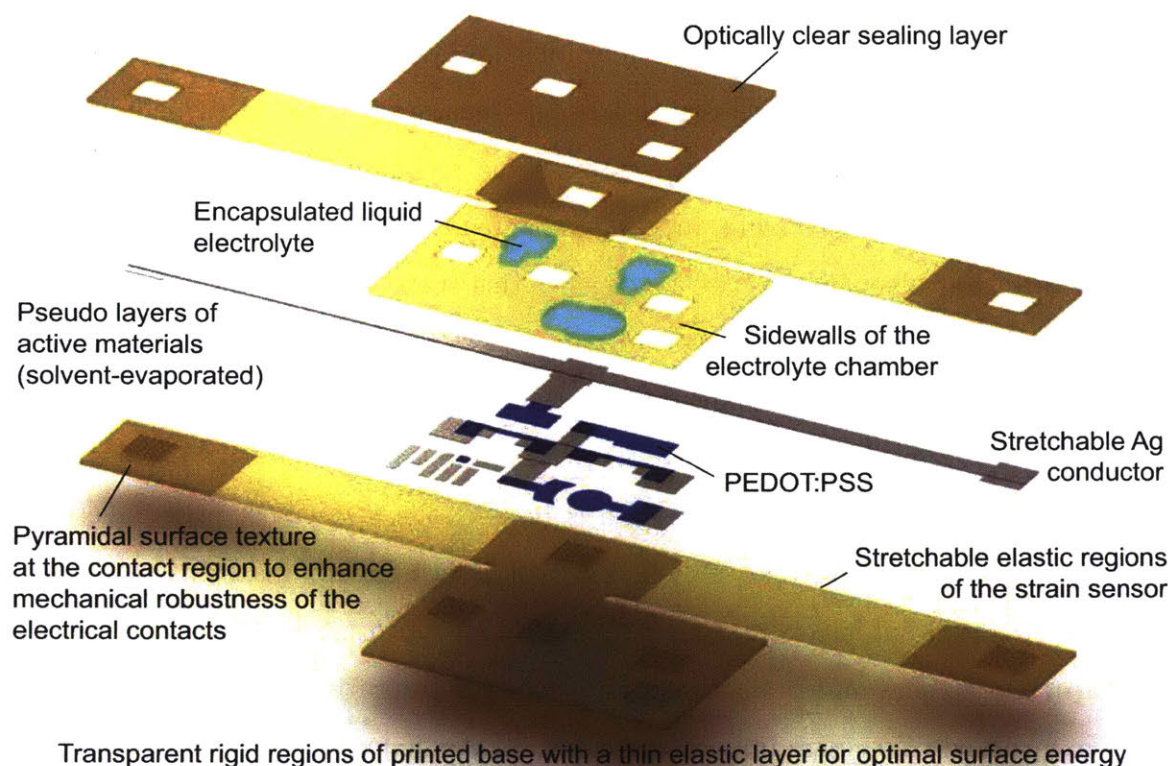
Figure 3-2: Schematic of the autonomous sensory composite. The composite is grouped into 4 sets of functional layers: a base with spatially varying mechanical stiffness and surface energy, electrical materials, electrolyte, and capping layers. All these materials are printed. The base is formed from droplets of UV curable acrylic polymer. Uppermost layers of the base consist of thin surface energy engineered elastic ELA layers to facilitate proper definition of solvent-based inks. Electrical contact regions of the base are textured with pyramids for mechanically robust contacts. Silver traces are obtained by precipitating silver from a liquid ink by local forced convection heating. The elastic matrix with silver nanoparticles forms a stretchable conductor. Thin poly(3,4-ethylenedioxythiophene) polystyrene sulfonate (PEDOT:PSS) layers are obtained by solvent evaporation and are used as the active semiconductor and electrochromic material. The printed conductive and semiconductor materials are capped by UV curable polymers and wells that hold the electrolyte, defining the active transistor geometry. The uppermost optically clear layer seals the electrolyte exposing only the electrical pads. This scheme shows the integration of elements with varying mechanical and dynamically-tunable electrical and optical properties in freeform architectures.
