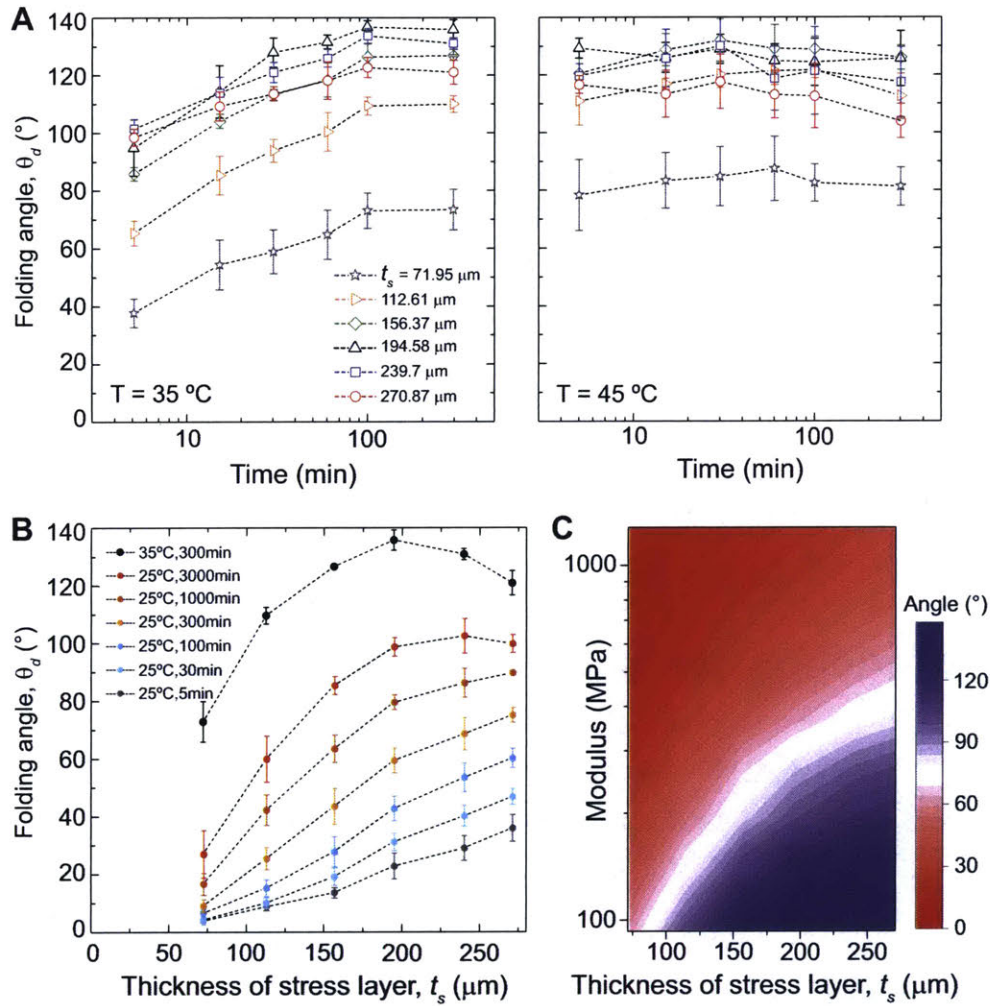
Figure 5-3: Bilayer characteristics at elevated temperatures and design guidelines A. Plots show the time dependence of the folding angle of the bilayer system used for creating folds at 35 °C and 45 °C. The folding angle shows little variation past 100 min at 35 °C. Samples approach a steady state folding angle after ~ 5 min at 45 °C. B. The folding angle is shown as a function of the stress layer thickness at various time instants at 25 °C. The black curve shows the saturated folding angle at 35 °C (after 300 min). Note that the optimum thickness of the stress layer for creating larger folds changes with time (due to a larger creep compliance). C. Finite element analysis (FEA) predictions of the folding angle based on geometry and time (or equivalently elastic modulus).
