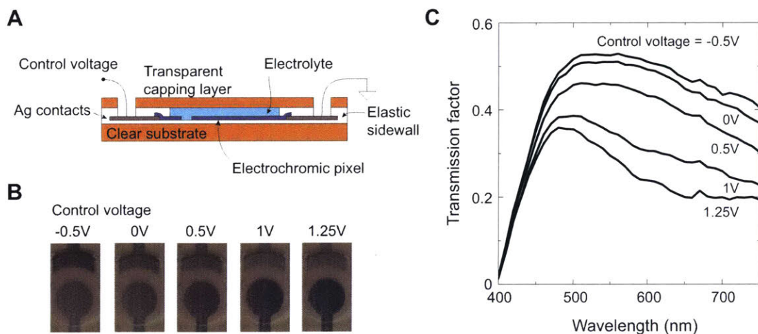
Figure 3-10: Electrochromic pixel. A. Cross sectional schematic of the electrochromic pixel. B. Optical images of the pixel as the voltage on the control electrode is cycled from -0.5 V to 1.25 V. The circular pixel is \sim 3 mm in size. C. Optical transmission through the pixel as a function of wavelength for different control voltages, normalized with respect to direct transmission through a 2 mm aperture.
