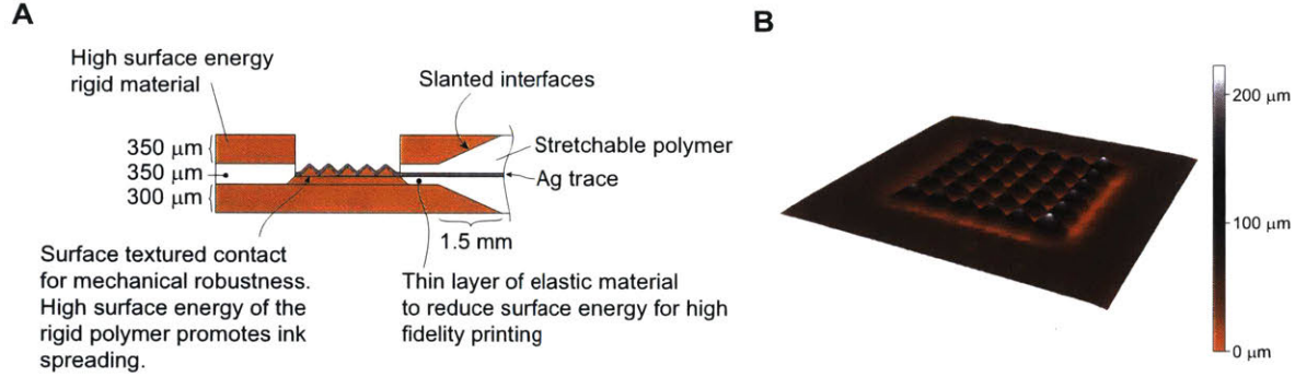
Figure 2-6: Textured contact. A. Schematic shows an electrical contact design in a printed device. The textured contact window and the slanted interfaces are of interest here. B. The height map of the textured contact measured using the Gelsight system.
