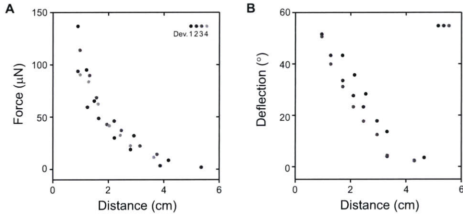
Figure 6-9: Force generated by our actuators. A. Blocking force generated by actuators with dimensions: t_p = 1 mm, \lambda = 0.15 , l_p = 9 mm, t_h = 0.25 mm, w_h = 0.5 mm, and l_h = 1 mm. The plot shows measurements from 4 identical devices, as a function of the distance between the device and the permanent magnet (Fig. 6-8C). B. Measured angular deflections for 3 identical devices.
